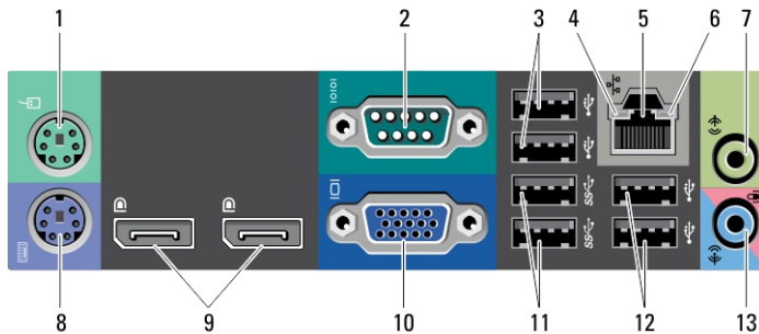
Angka 4. Tampilan Panel Belakang Small Form Factor
